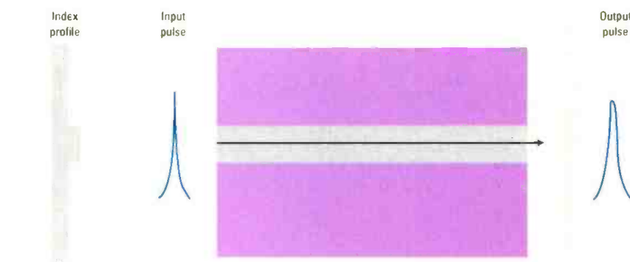
Figure 9. A single-mode fiber (mono mode) only allows one ray/mode to propagate through the fiber. This is done by shrinking the fiber core to comparable dimensions of the transmitted wavelength.
