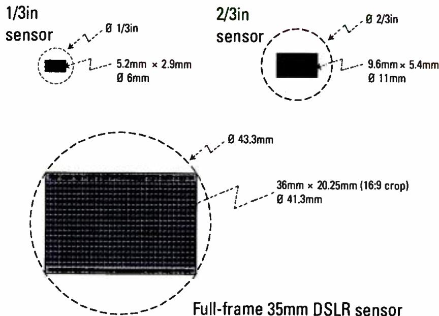
Figure 1. Shown here are dimensions of various sensors, to scale.
